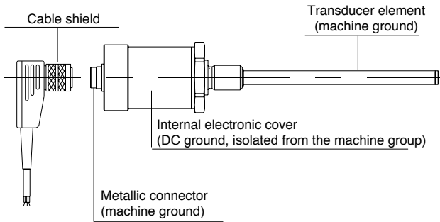
Connector output IK4-A-A/B/C/H
